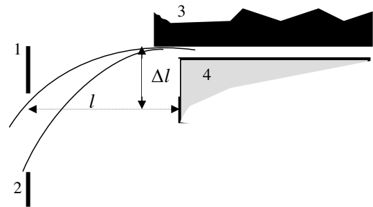
Fig. 3. Schematic view of the integral method for measuring the neutron horizontal velocity component spectrum along the neutron beam axis and for shaping this spectrum. The black vertical lines on the left show the upper plate (1) and the lower plate (2) of the entrance collimator. Each plate could be adjusted to the required height. The jagged black rectangle on the top indicates a scatterer (3); the incomplete grey rectangle below shows the mirror (4). The distance between the entry collimator and mirror is equal to l . The neutron trajectory rises by \Delta l at the horizontal length l . The neutron trajectory is horizontal at the entrance to the mirror/scatterer slit
