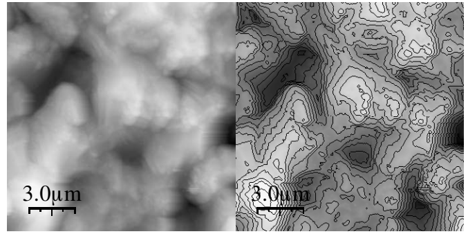
Fig. 2. A typical surface profile of a scatterer with a copper coating, measured using an atomic-force microscope. The maximum height difference between two points here is equal to 2 \mu\text{m} , the distance between neighbouring “hills” is 7 \mu\text{m} .
